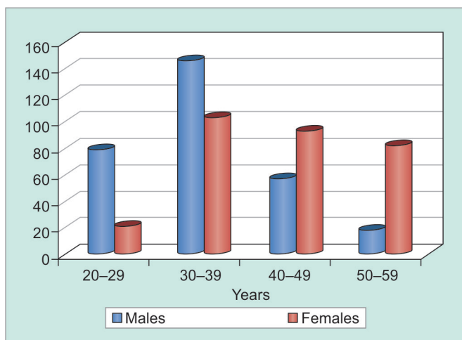
Graph 1: Age-wise distribution of the patients
