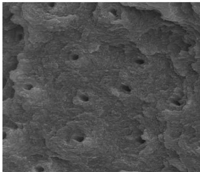
Fig. 4: Absence of smear layer on dentin irradiated with Er:YAG laser (pulse energy of 200 mJ for 2 seconds, focused, noncontact mode, cooling to 0.14 ml/seconds, Twinlight, Fotona Medical Lasers, Ljubljana, Slovenia) (Magnification at 3000x)
