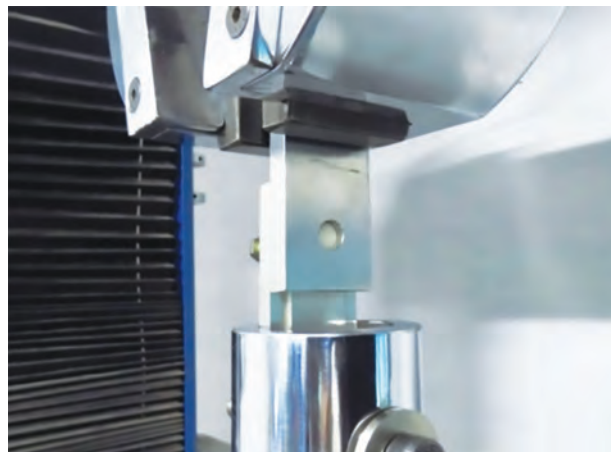
Fig. 5: Jig with test sample in situ
